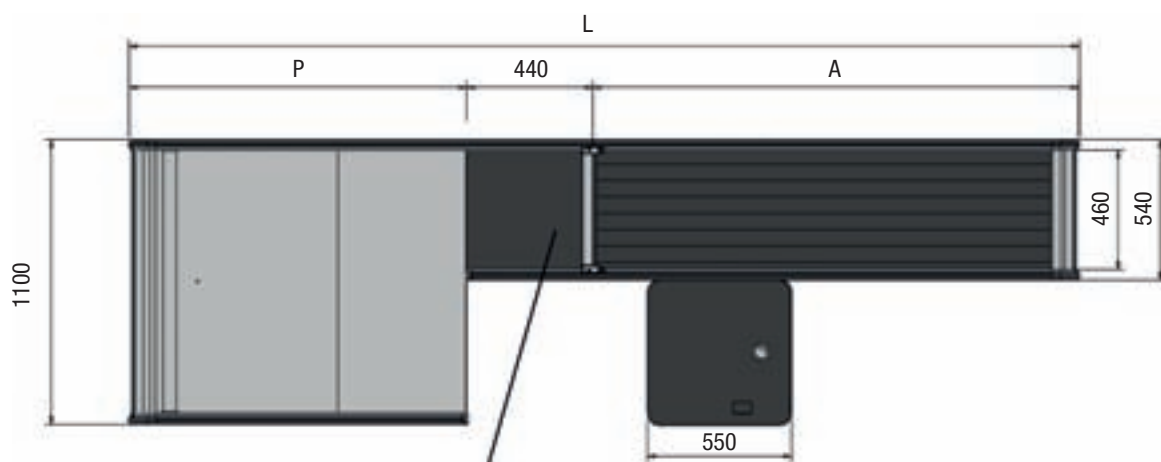
Pianetto scanner/Scanner Shelf: 362x460 P (mm)
