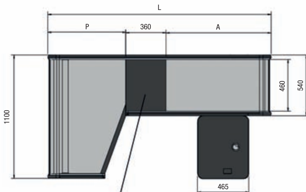
Pianetto scanner/Scanner Shelf: 360x460 P (mm)
